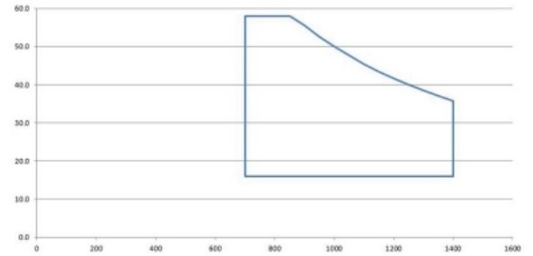
Operating frequency graph
