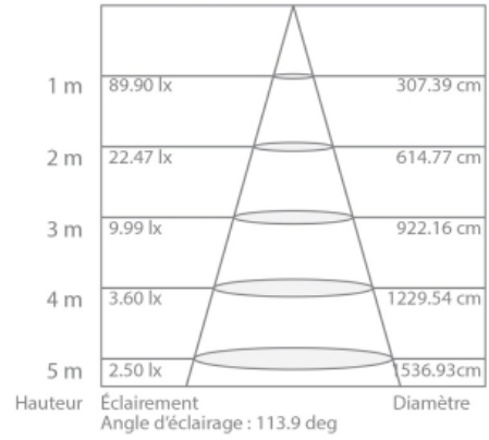
Courbe lux - distance
