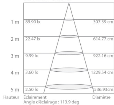
Courbe lux - distance
